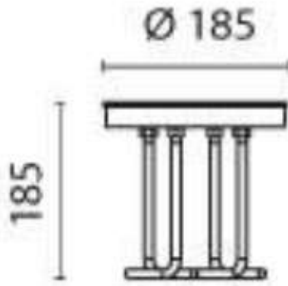
ANCHOR FLANGE
